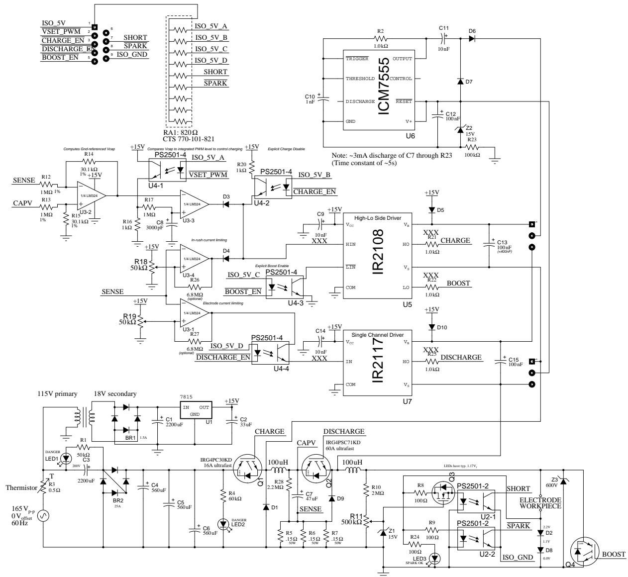
'GARDEN OF EDM' POWER SUPPLY ~50A, ~300VDC. Designed by C. Scott Ananian (edm@cscott.net)
